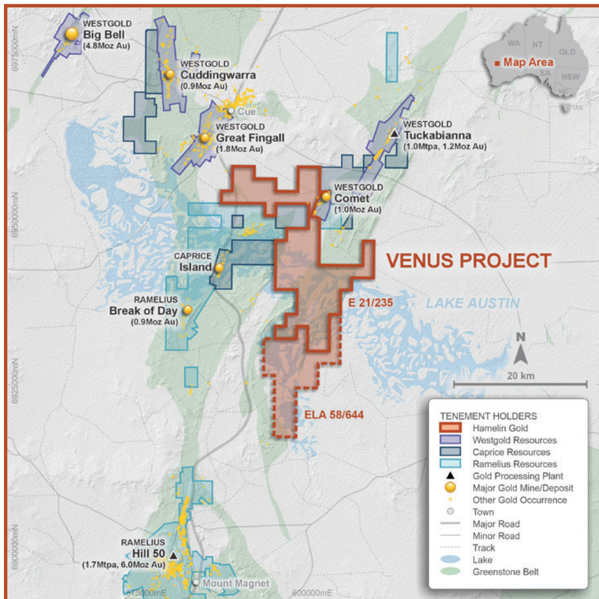
Figure 8 – Venus Project Location Map, Key tenement holders and gold occurrences
