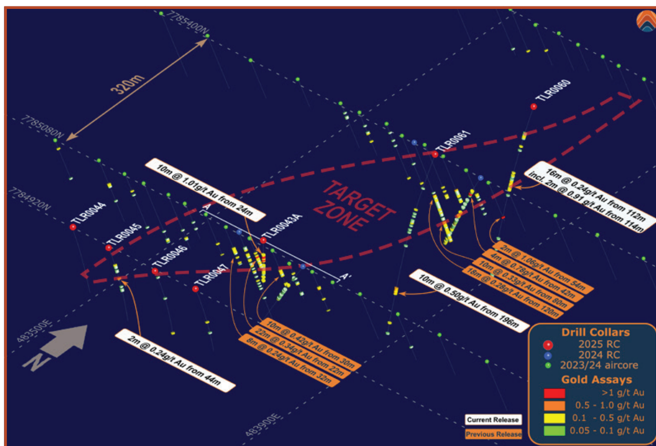
Figure 7 – Fremlins South Isometric view to the northwest
