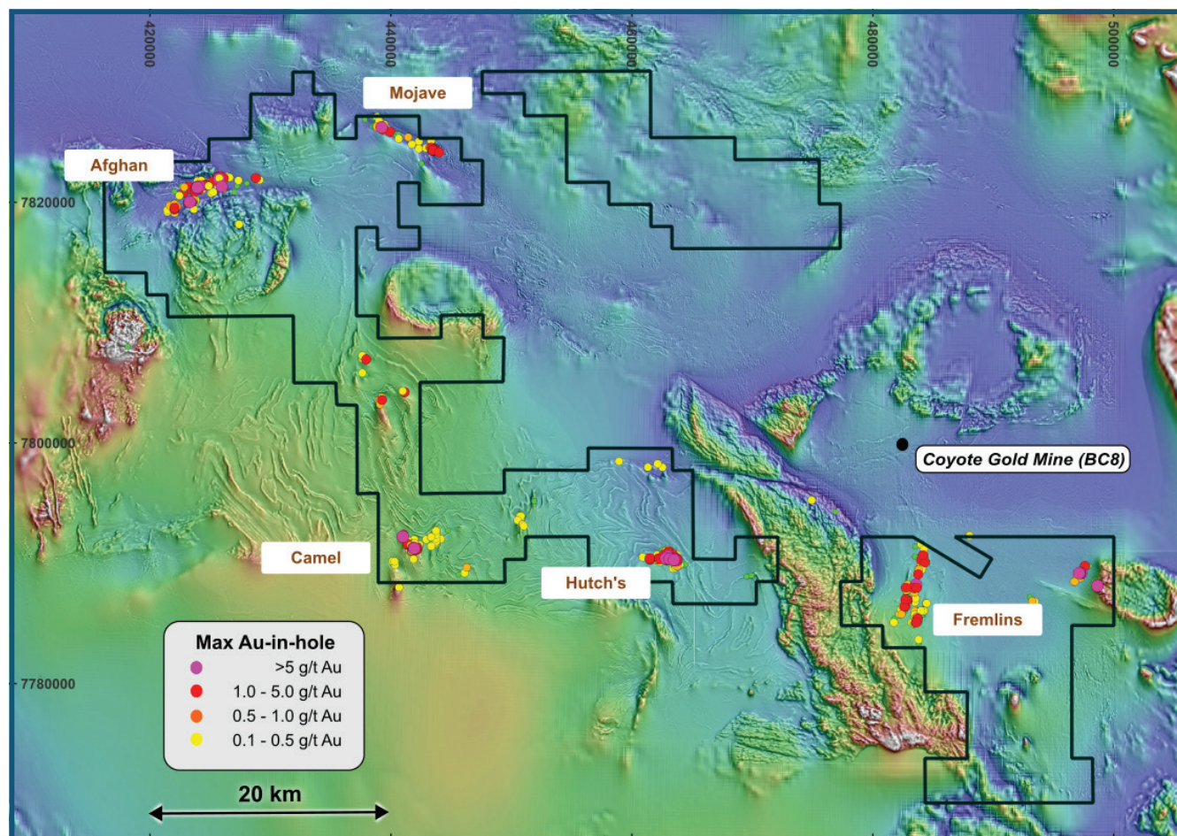
Figure 3 - West Tanami Max Gold-in-hole plan (>0.1g/t Au)
