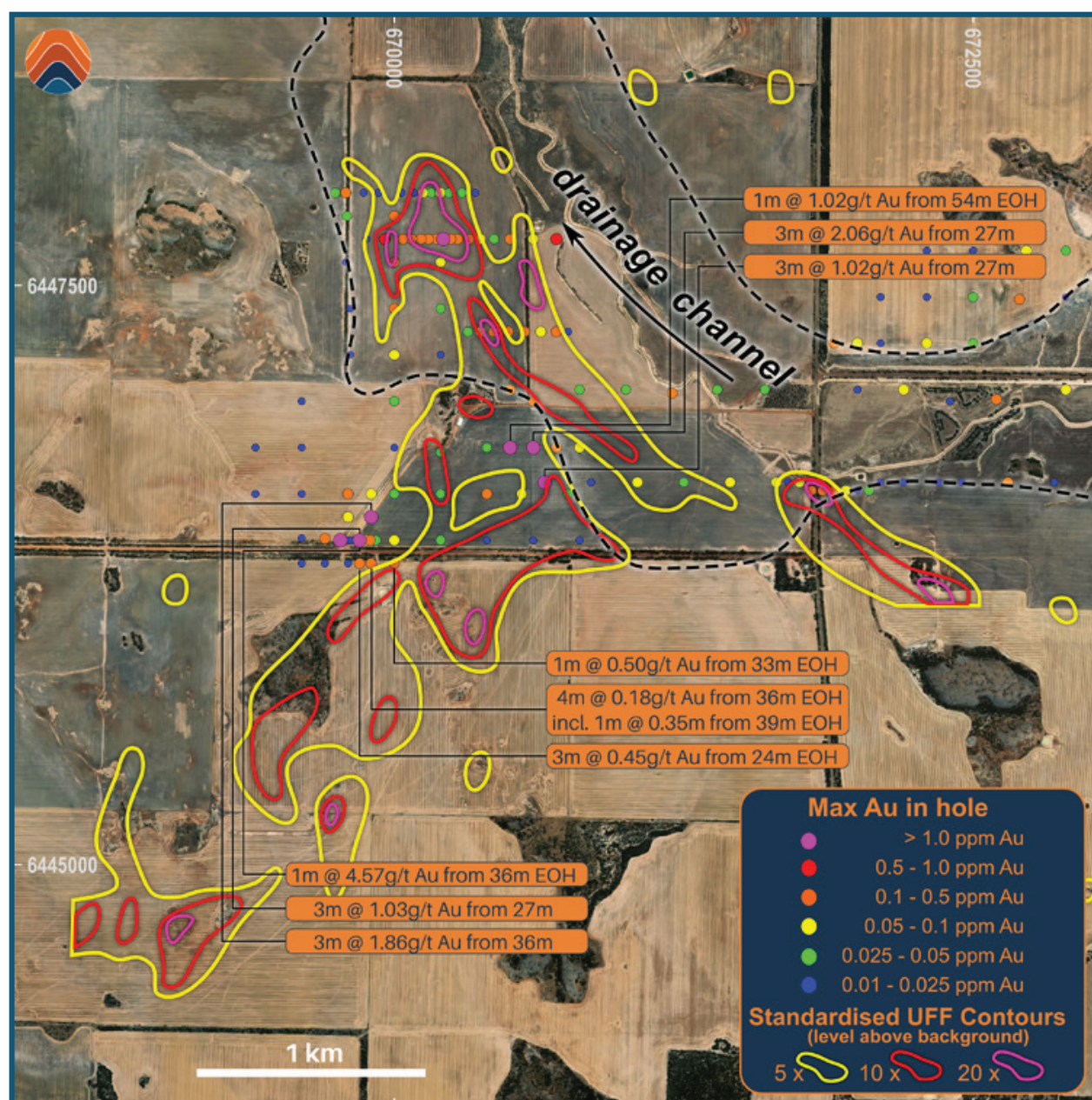
Figure 10 – Anderson project Geochemical anomalies, historical drillhole locations on Bing satellite imagery
