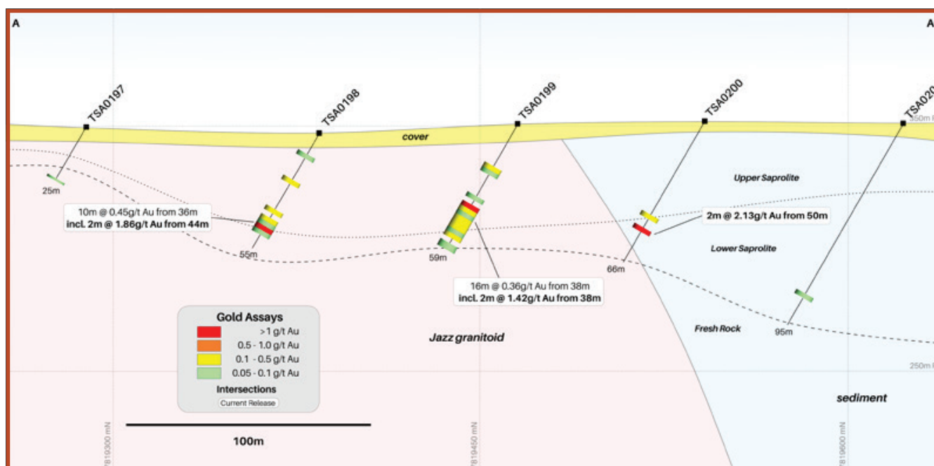
Figure 5 – Jazz Prospect Aircore drill cross section 422,020mE
