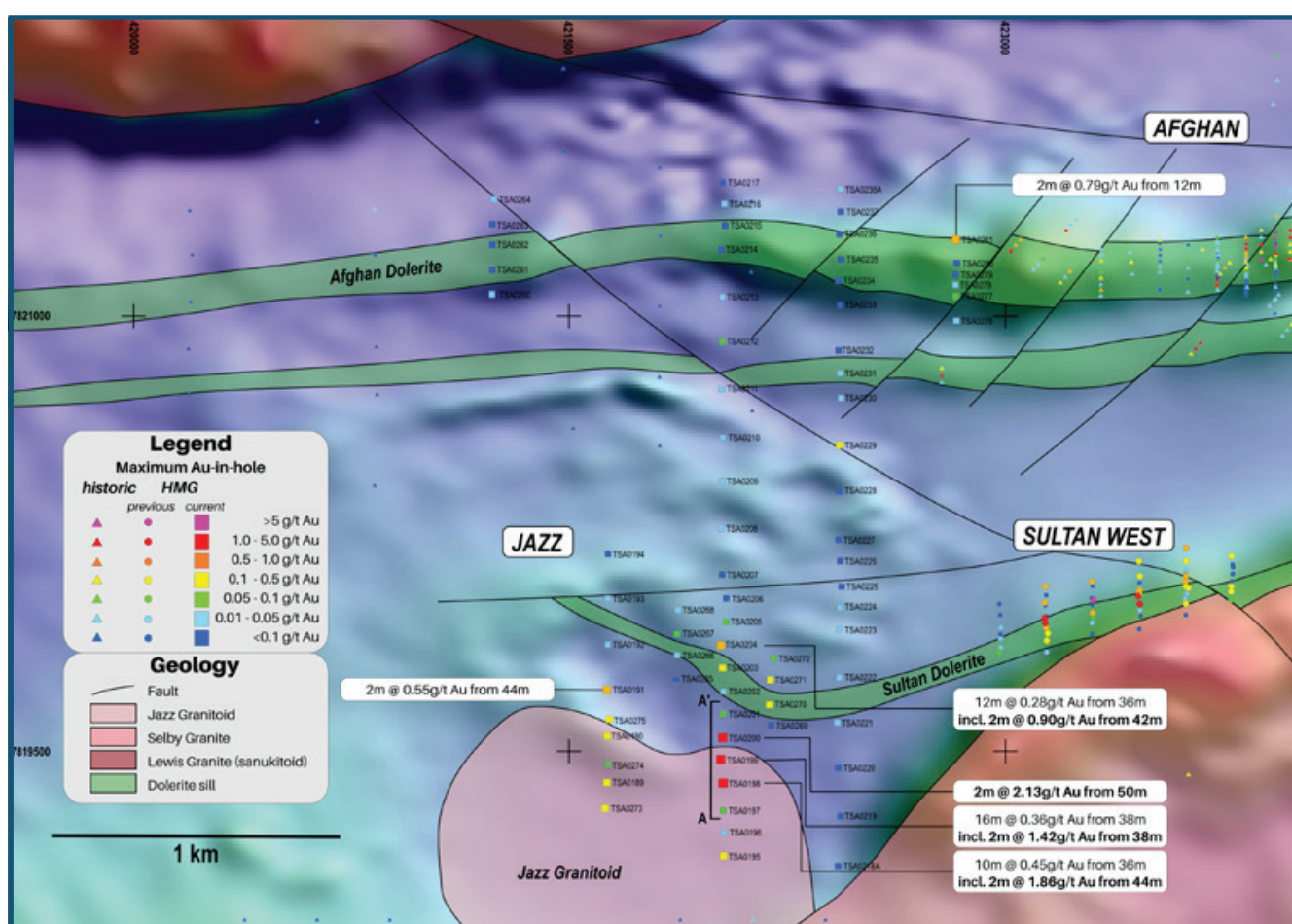
Figure 4 – Jazz Prospect Aircore drillhole location plan on magnetics
