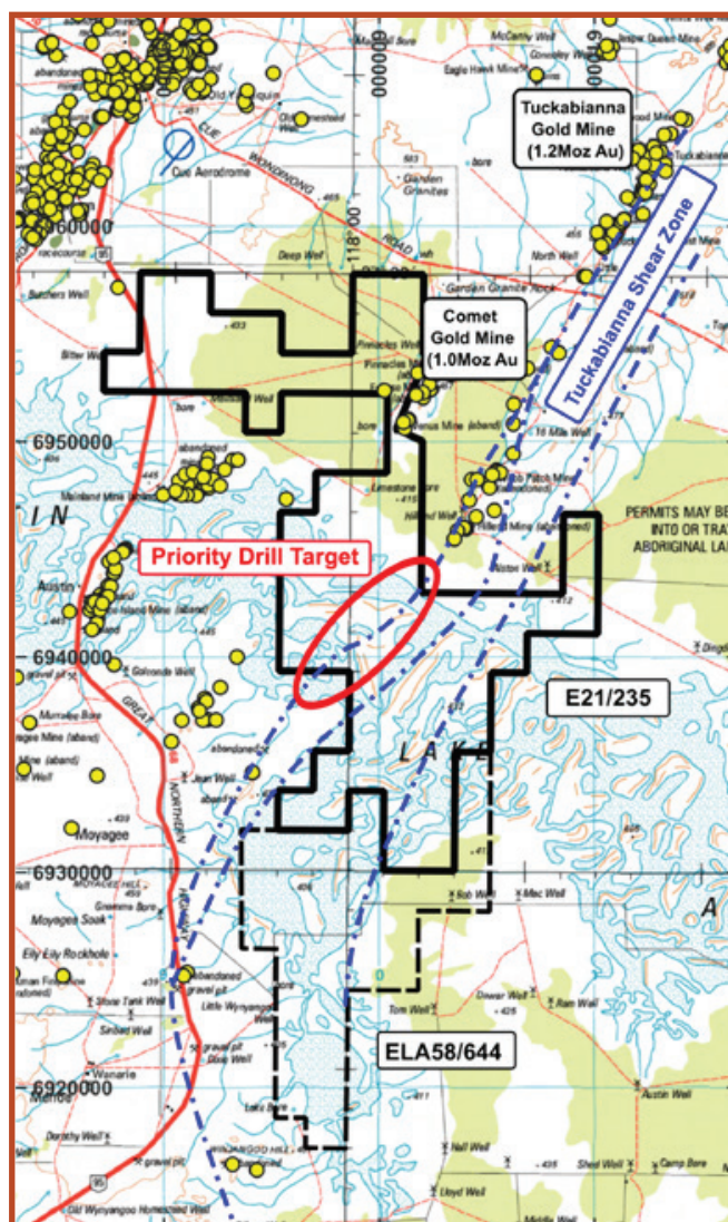
Figure 9b – Venus Project Leasing, structural interpretation and Priority drill target
