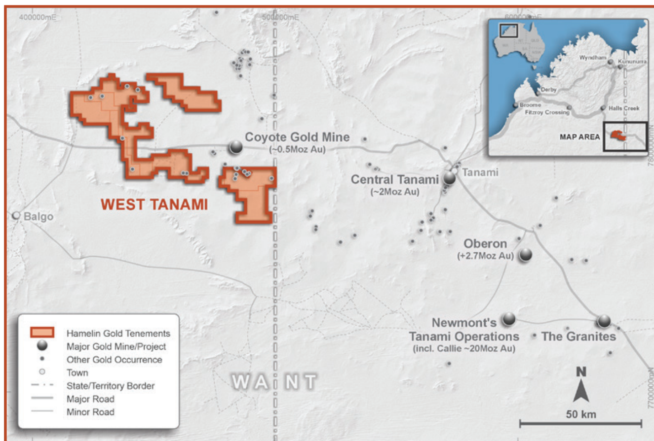
Figure 2 - West Tanami Regional Project Location Map
