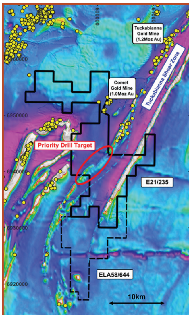
Figure 9a – Venus Project Leasing, gold occurrences on magnetics
